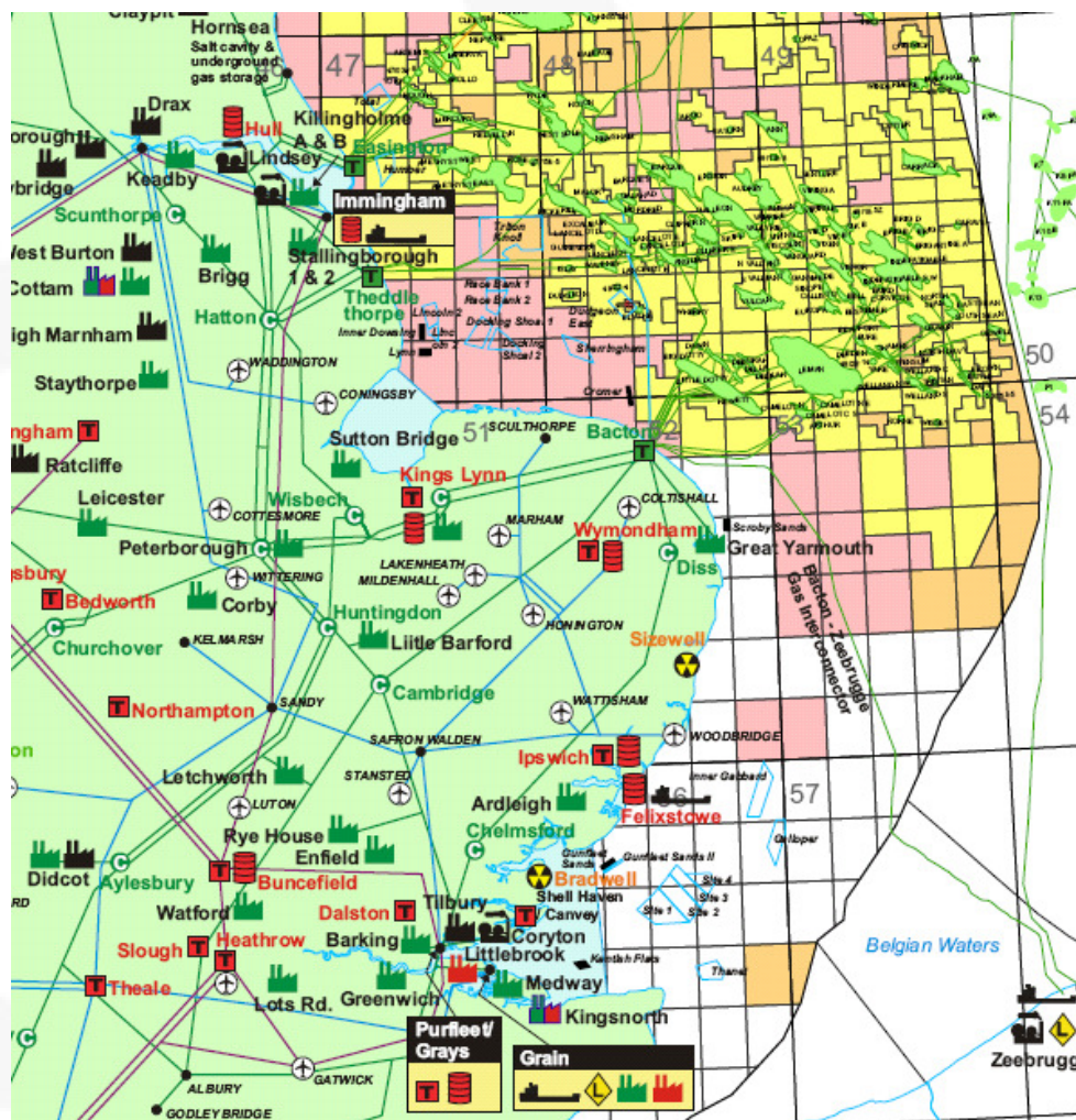
CO 2 sources in and around the East of England
